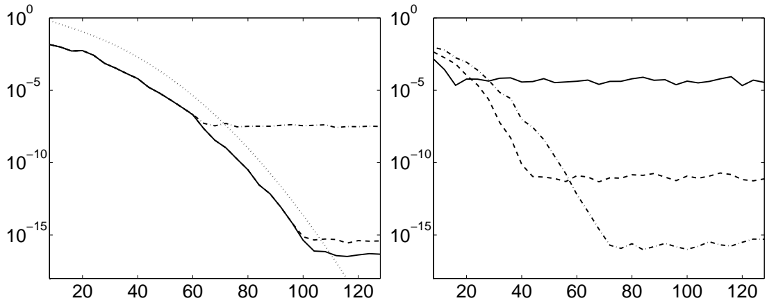
Figure 4.1: Error E_\infty for n = 8, 12, 16, \dots, 128 and N = M = 1000 .
